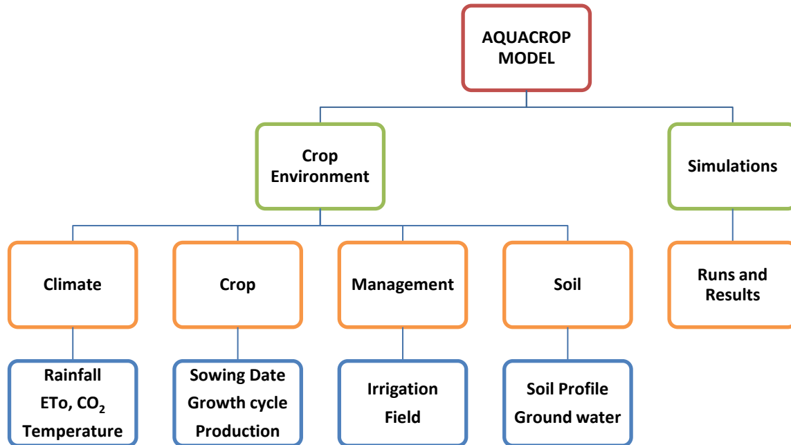
Figure 5.1 Shows the framework of the aquacrop model adopted from (FAO, Aquacrop, 2016)
